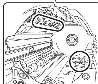
Paper separation hook
